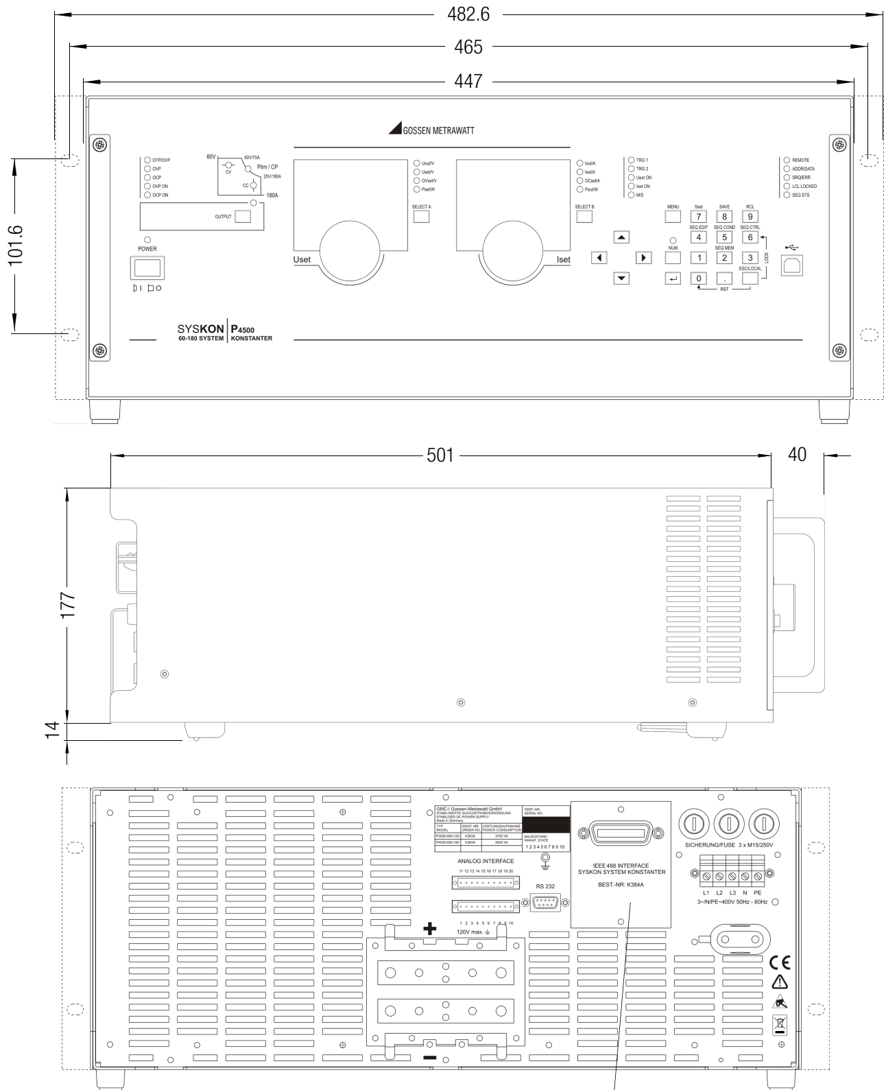
Dimensional Drawing SYSKON P3000 / P4500
