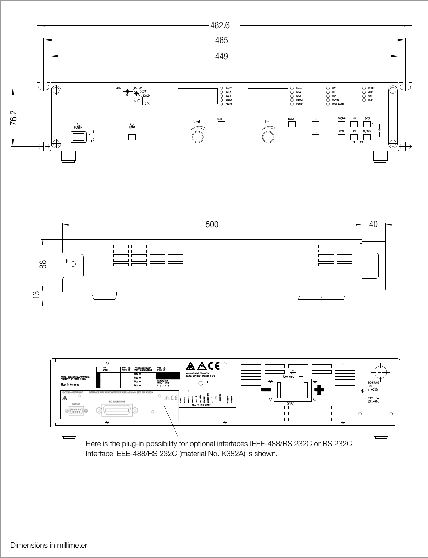
Dimensional Drawing
