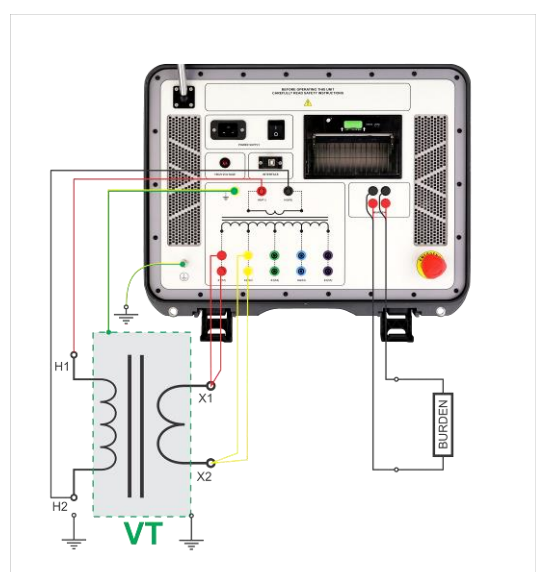
Connecting CVA500 to a VT – secondary winding resistance test and insulation resistance test
