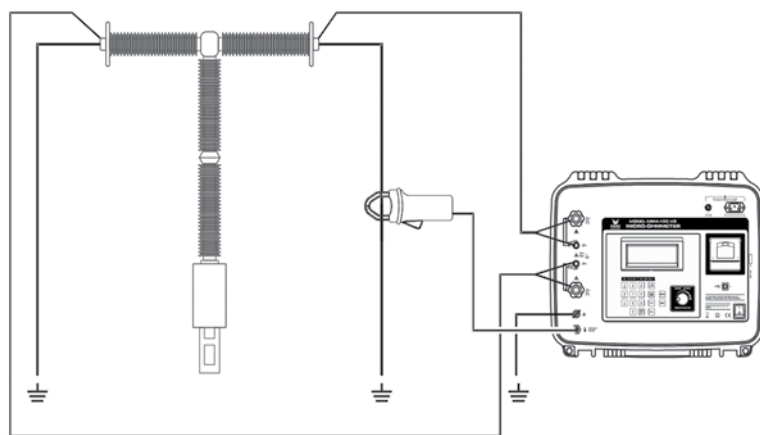
Double Ground Test Measurement Set-up for increased safety in substations
